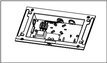
4. Fix mounting bracket to wall.
